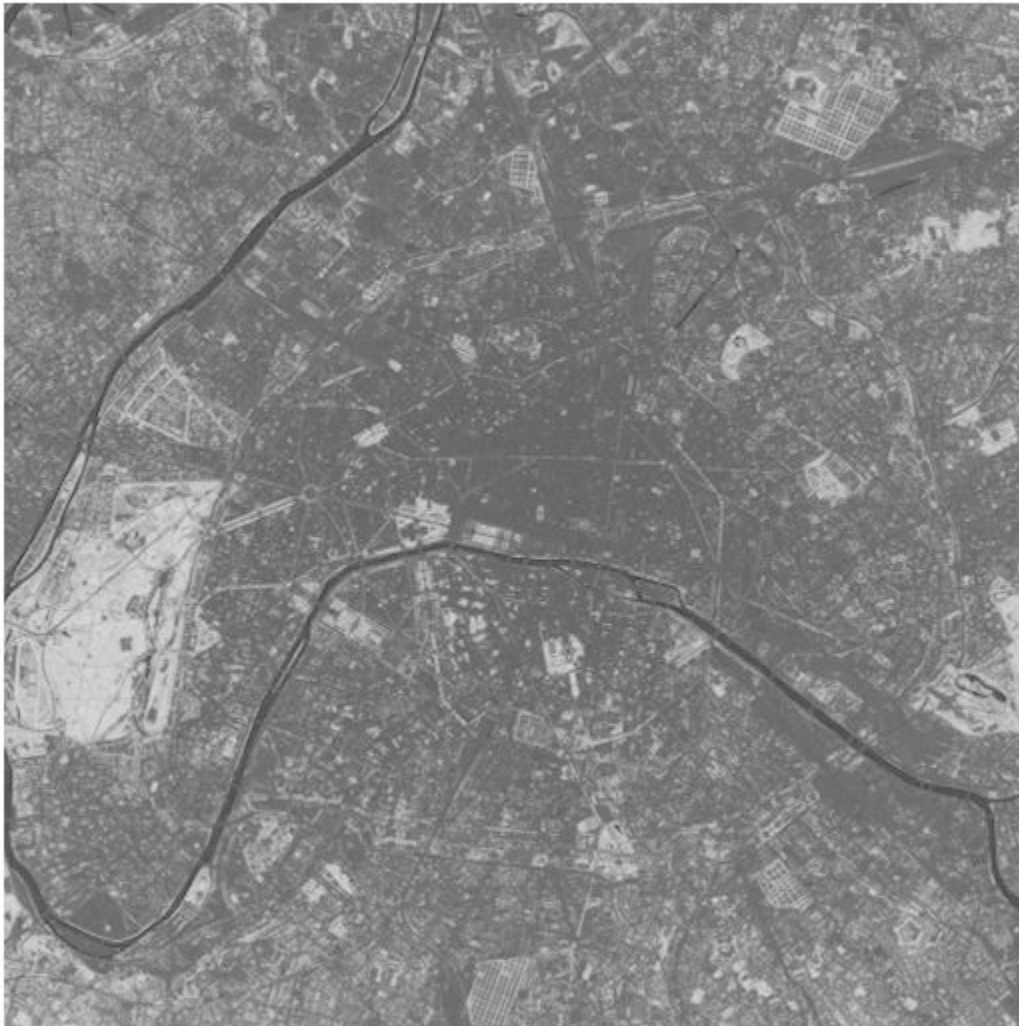
Normalized Difference Vegetation Index
