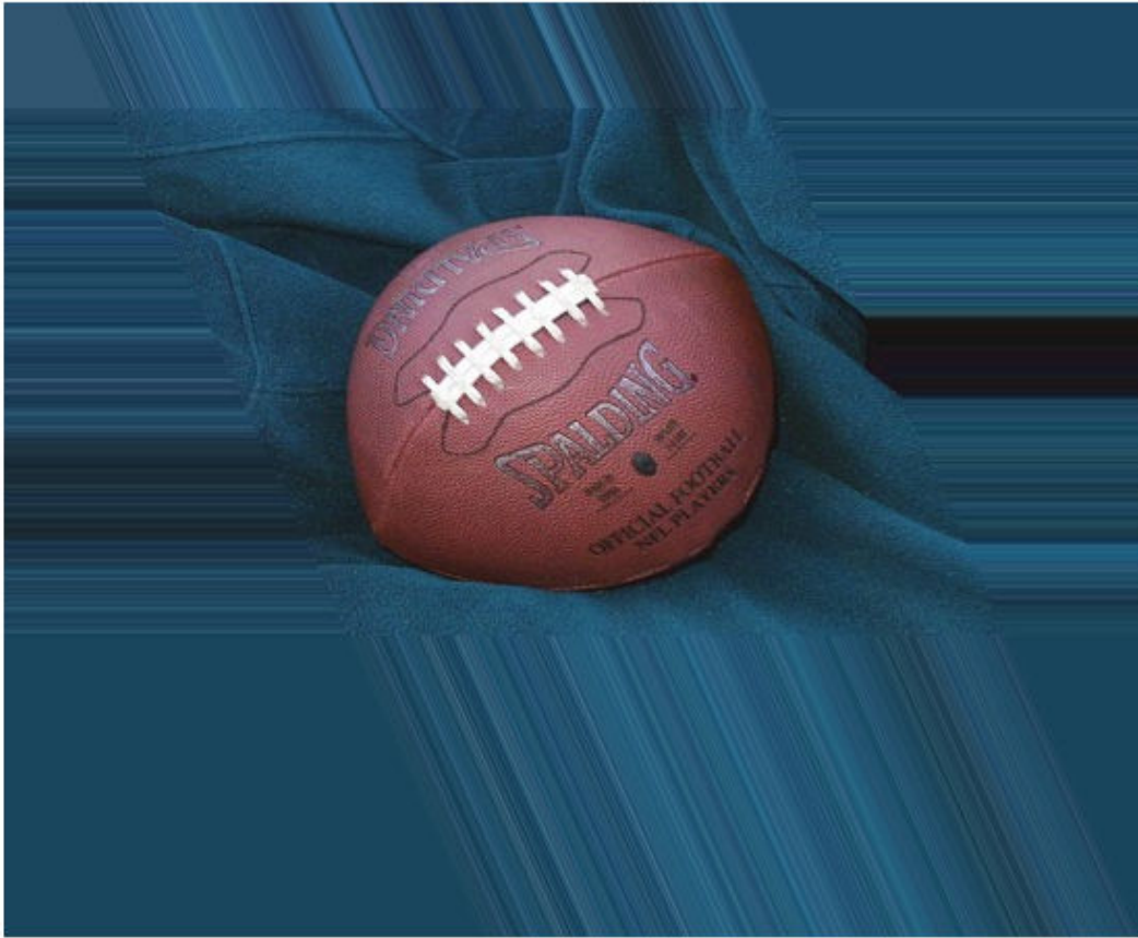
Pad Method = 'replicate'
